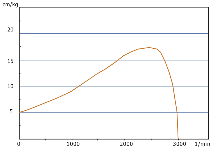
CURVA MOTOR A 240 V.
